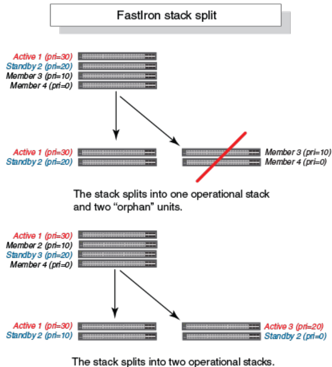
FIGURE 43 Hitless Stacking Support in a Stack Split
