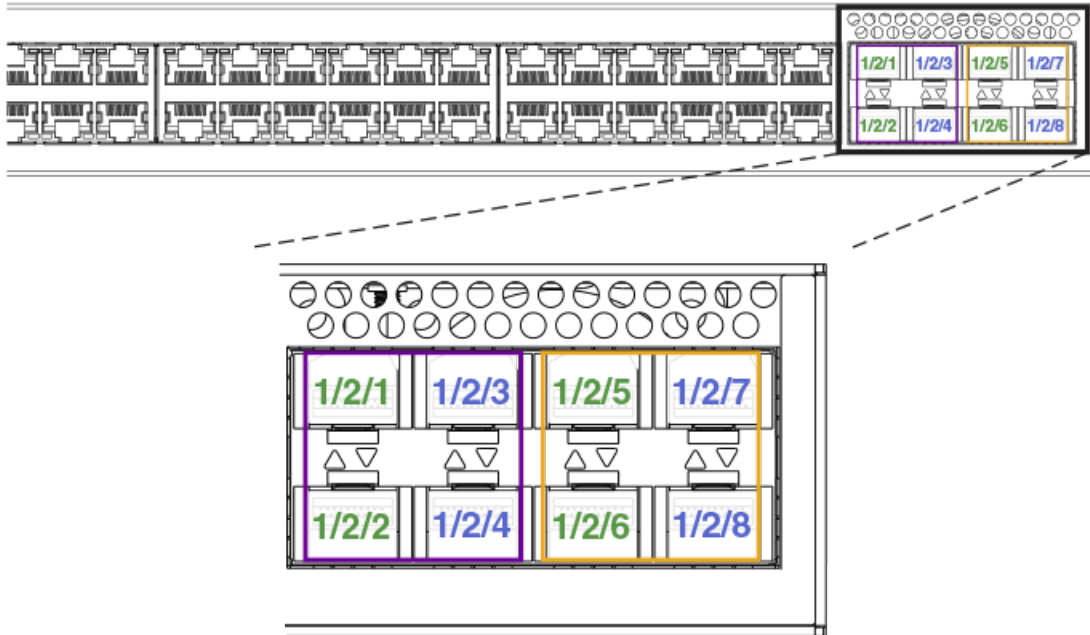
FIGURE 13 ICX 7250 Stacking Ports
