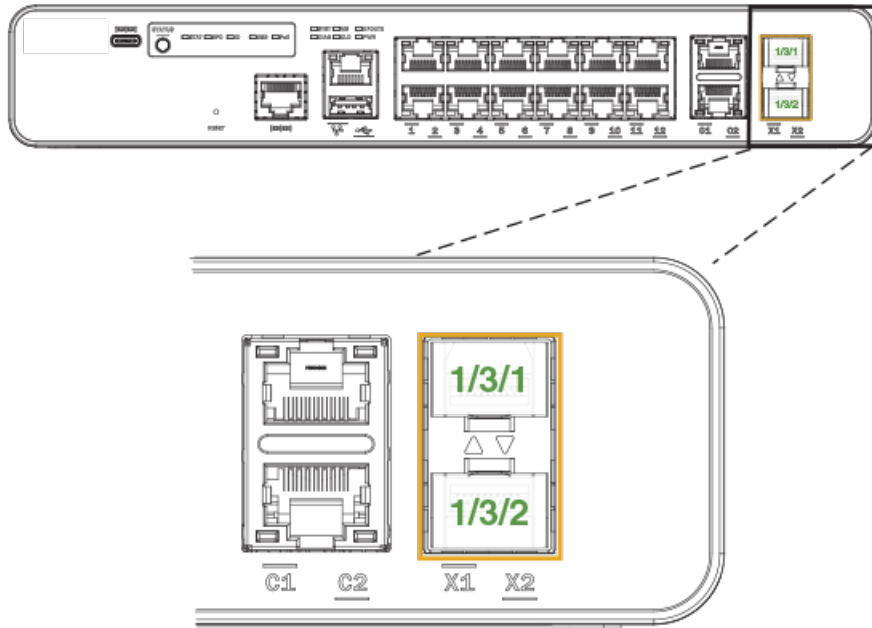
FIGURE 3 ICX 7150-C12P Stacking Ports
